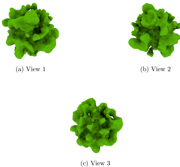
Figure 4: Isosurface at threshold=0.512000. Views generated by ChimeraX at a the following X, Y, Z angles: View 1 (0, -90, -90), View 2 (-90, 0, -90), View 3 (0, 0, 0).
