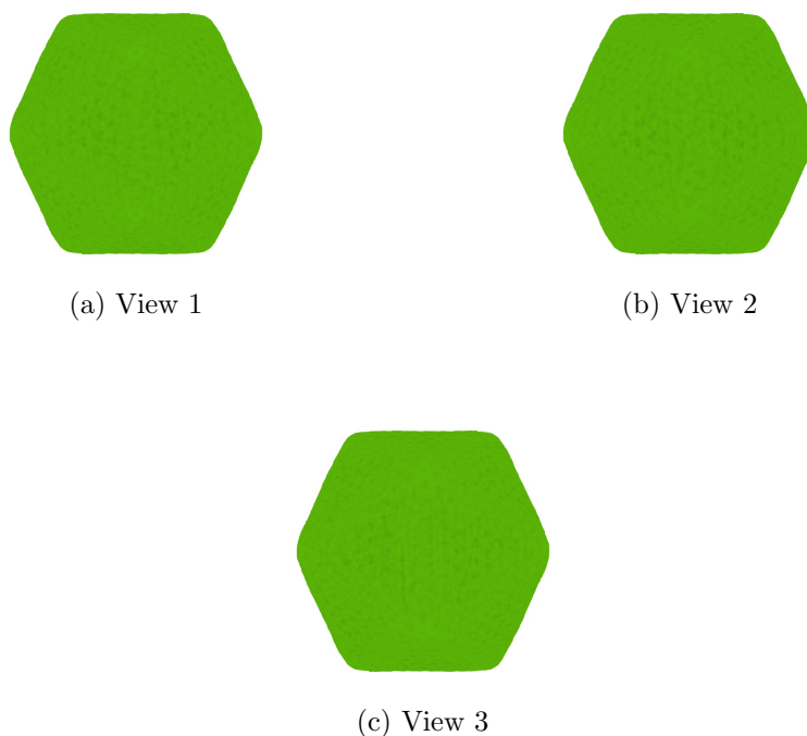
Figure 4: Isosurface at threshold=1.680000. Views generated by ChimeraX at a the following X, Y, Z angles: View 1 (0, -90, -90), View 2 (-90, 0, -90), View 3 (0, 0, 0).
