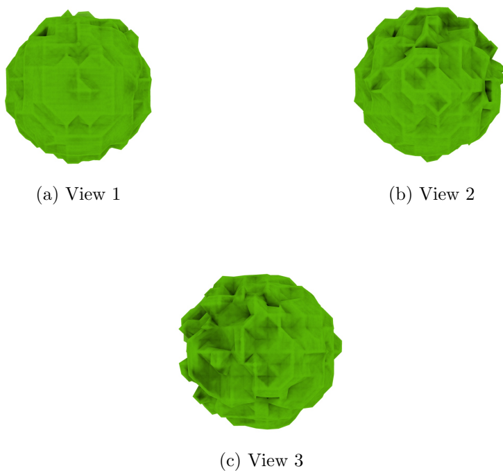
Figure 4: Isosurface at threshold=0.129000. Views generated by ChimeraX at a the following X, Y, Z angles: View 1 (0, -90, -90), View 2 (-90, 0, -90), View 3 (0, 0, 0).
