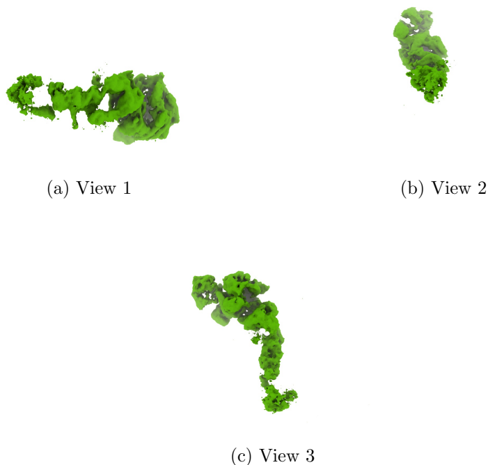
Figure 4: Isosurface at threshold=0.008000. Views generated by ChimeraX at a the following X, Y, Z angles: View 1 (0, -90, -90), View 2 (-90, 0, -90), View 3 (0, 0, 0).
