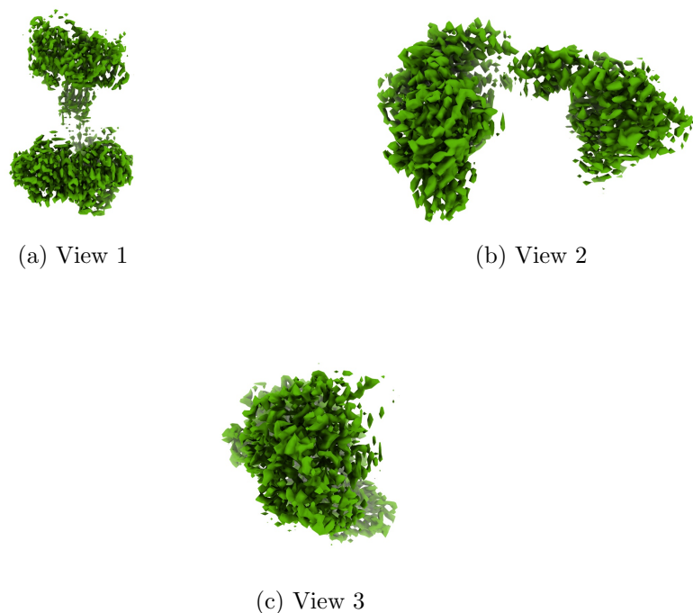
Figure 4: Isosurface at threshold=0.869000. Views generated by ChimeraX at a the following X, Y, Z angles: View 1 (0, -90, -90), View 2 (-90, 0, -90), View 3 (0, 0, 0).
