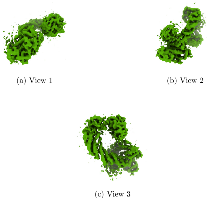
Figure 4: Isosurface at threshold=0.055000. Views generated by ChimeraX at a the following X, Y, Z angles: View 1 (0, -90, -90), View 2 (-90, 0, -90), View 3 (0, 0, 0).
