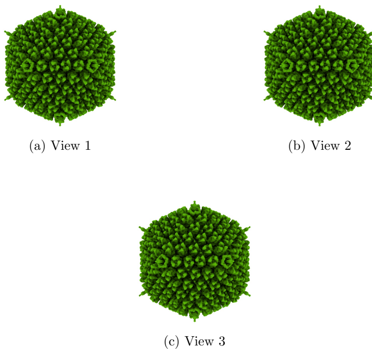
Figure 4: Isosurface at threshold=76.500000. Views generated by ChimeraX at a the following X, Y, Z angles: View 1 (0, -90, -90), View 2 (-90, 0, -90), View 3 (0, 0, 0).
