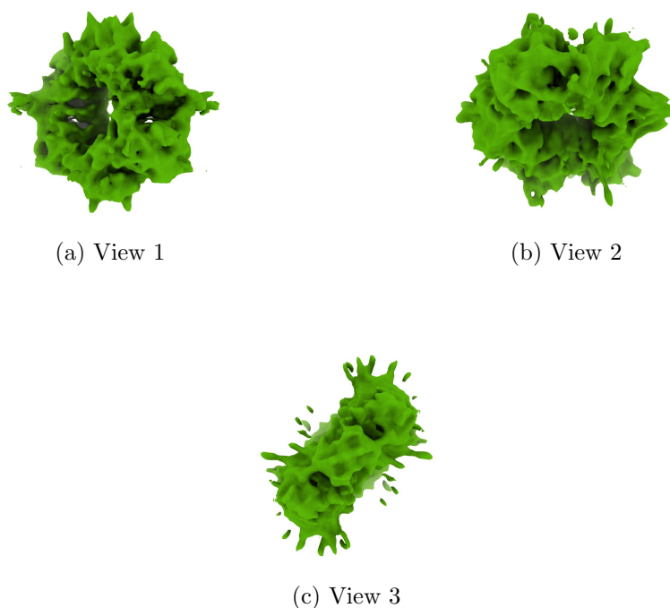
Figure 4: Isosurface at threshold=0.255000. Views generated by ChimeraX at a the following X, Y, Z angles: View 1 (0, -90, -90), View 2 (-90, 0, -90), View 3 (0, 0, 0).
