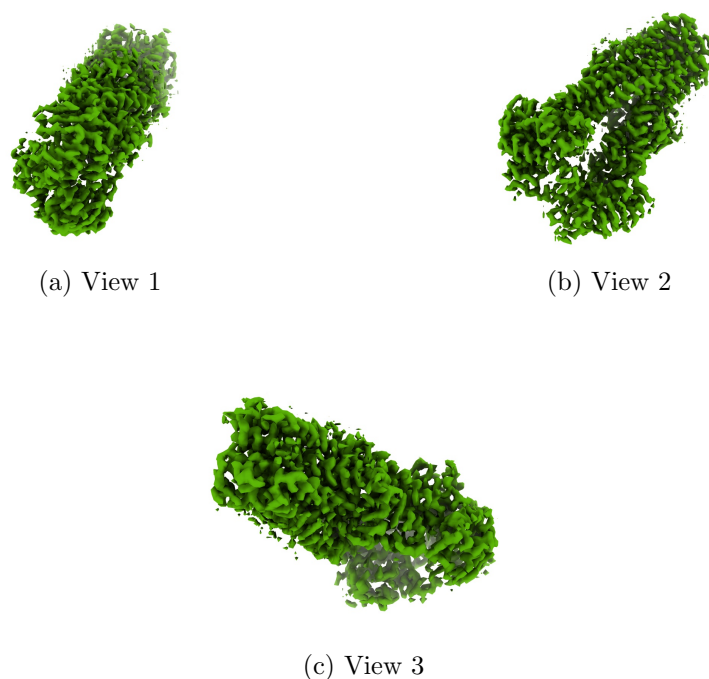
Figure 4: Isosurface at threshold=0.038000. Views generated by ChimeraX at a the following X, Y, Z angles: View 1 (0, -90, -90), View 2 (-90, 0, -90), View 3 (0, 0, 0).
