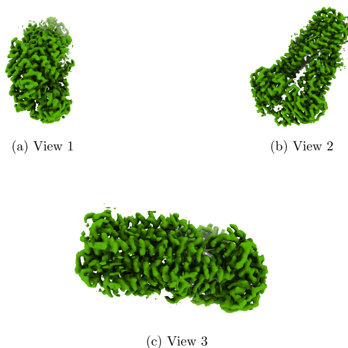
Figure 4: Isosurface at threshold=0.030000. Views generated by ChimeraX at a the following X, Y, Z angles: View 1 (0, -90, -90), View 2 (-90, 0, -90), View 3 (0, 0, 0).
