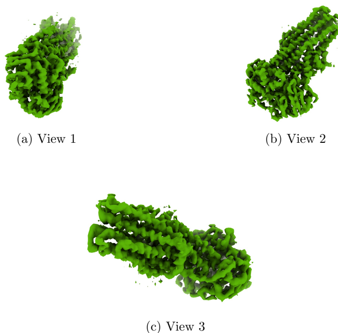
Figure 4: Isosurface at threshold=0.024000. Views generated by ChimeraX at a the following X, Y, Z angles: View 1 (0, -90, -90), View 2 (-90, 0, -90), View 3 (0, 0, 0).
