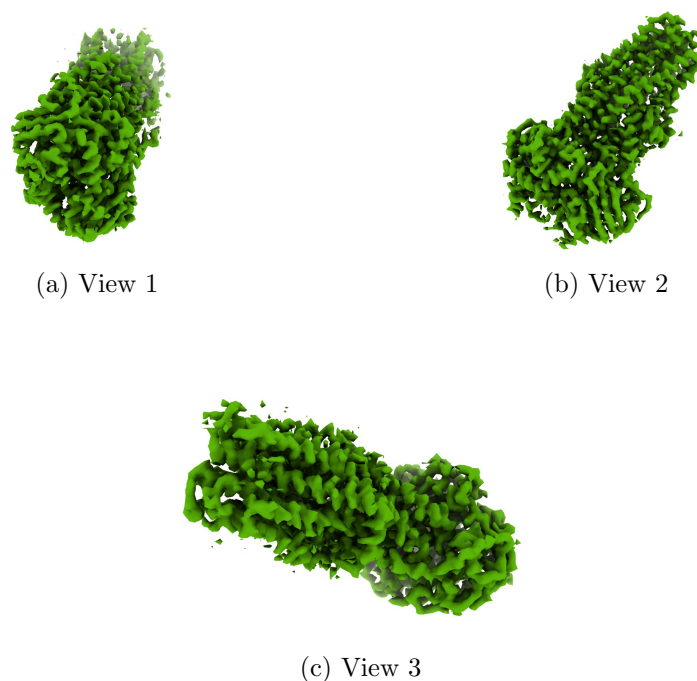
Figure 4: Isosurface at threshold=0.027500. Views generated by ChimeraX at the following X, Y, Z angles: View 1 (0, -90, -90), View 2 (-90, 0, -90), View 3 (0, 0, 0).
