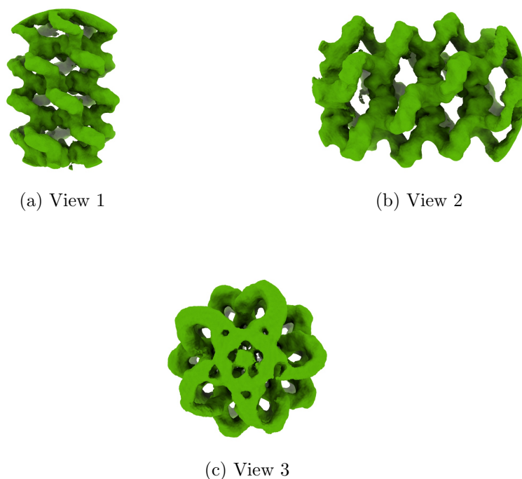
Figure 4: Isosurface at threshold=0.002700. Views generated by ChimeraX at a the following X, Y, Z angles: View 1 (0, -90, -90), View 2 (-90, 0, -90), View 3 (0, 0, 0).
