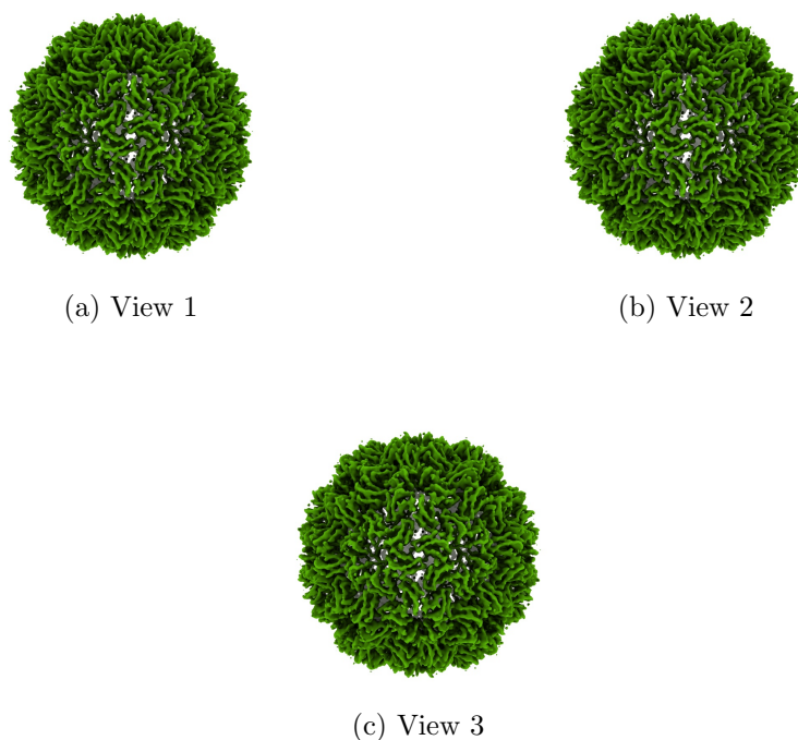
Figure 4: Isosurface at threshold=0.115000. Views generated by ChimeraX at the following X, Y, Z angles: View 1 (0, -90, -90), View 2 (-90, 0, -90), View 3 (0, 0, 0).
