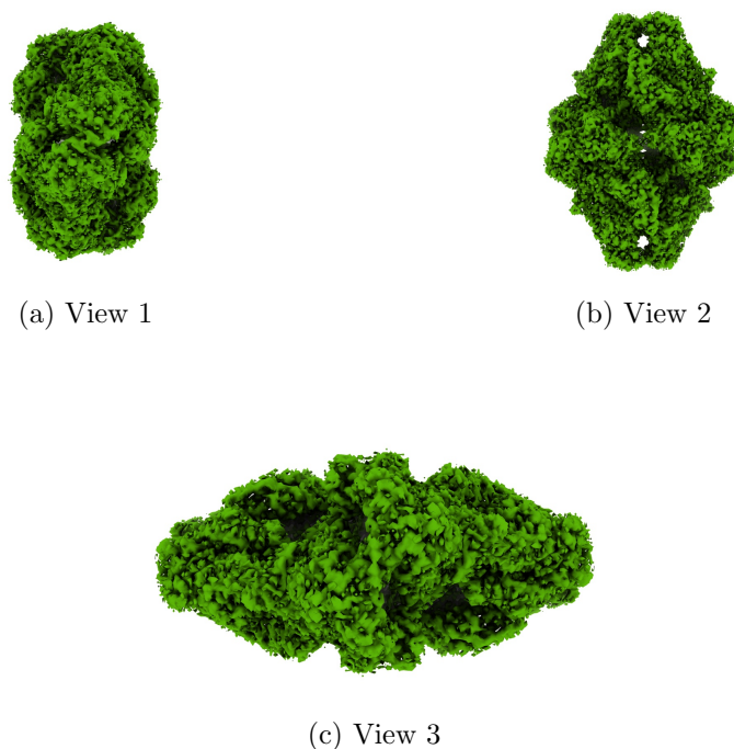
Figure 4: Isosurface at threshold=0.006890. Views generated by ChimeraX at a the following X, Y, Z angles: View 1 (0, -90, -90), View 2 (-90, 0, -90), View 3 (0, 0, 0).
