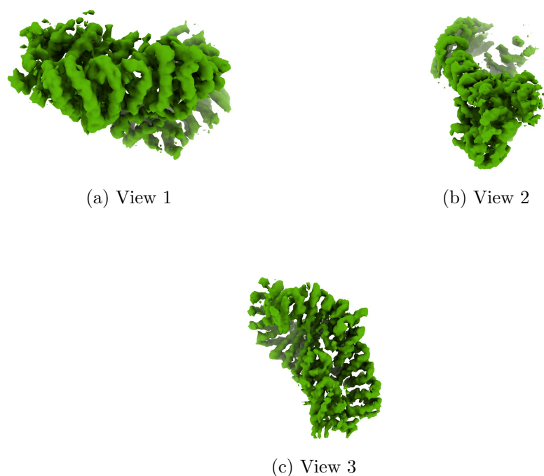
Figure 4: Isosurface at threshold=0.690000. Views generated by ChimeraX at a the following X, Y, Z angles: View 1 (0, -90, -90), View 2 (-90, 0, -90), View 3 (0, 0, 0).
