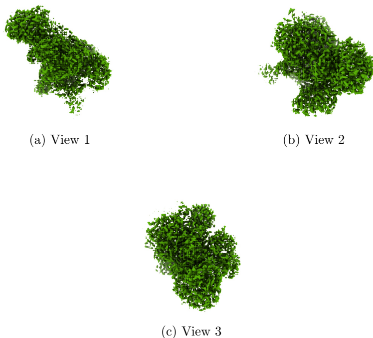
Figure 4: Isosurface at threshold=0.127000. Views generated by ChimeraX at a the following X, Y, Z angles: View 1 (0, -90, -90), View 2 (-90, 0, -90), View 3 (0, 0, 0).
