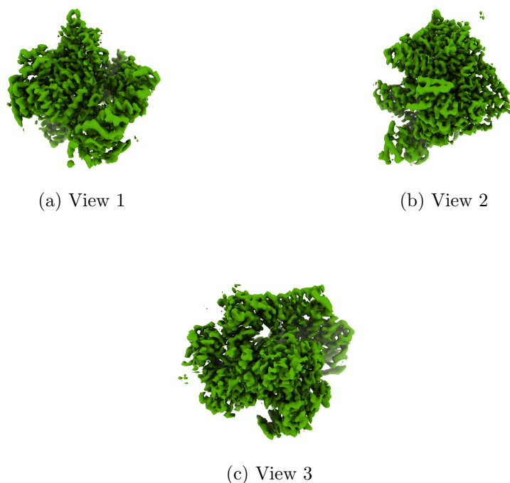
Figure 4: Isosurface at threshold=0.780000. Views generated by ChimeraX at a the following X, Y, Z angles: View 1 (0, -90, -90), View 2 (-90, 0, -90), View 3 (0, 0, 0).
