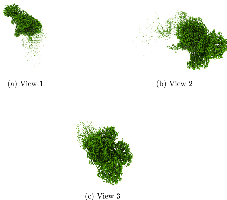
Figure 4: Isosurface at threshold=0.120000. Views generated by ChimeraX at the following X, Y, Z angles: View 1 (0, -90, -90), View 2 (-90, 0, -90), View 3 (0, 0, 0).
