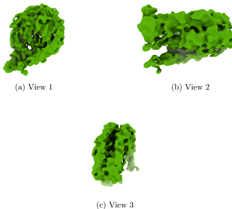
Figure 4: Isosurface at threshold=0.009600. Views generated by ChimeraX at a the following X, Y, Z angles: View 1 (0, -90, -90), View 2 (-90, 0, -90), View 3 (0, 0, 0).
