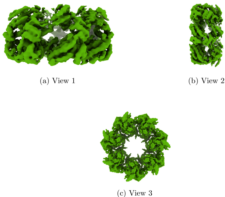
Figure 4: Isosurface at threshold=0.017200. Views generated by ChimeraX at the following X, Y, Z angles: View 1 (0, -90, -90), View 2 (-90, 0, -90), View 3 (0, 0, 0).
