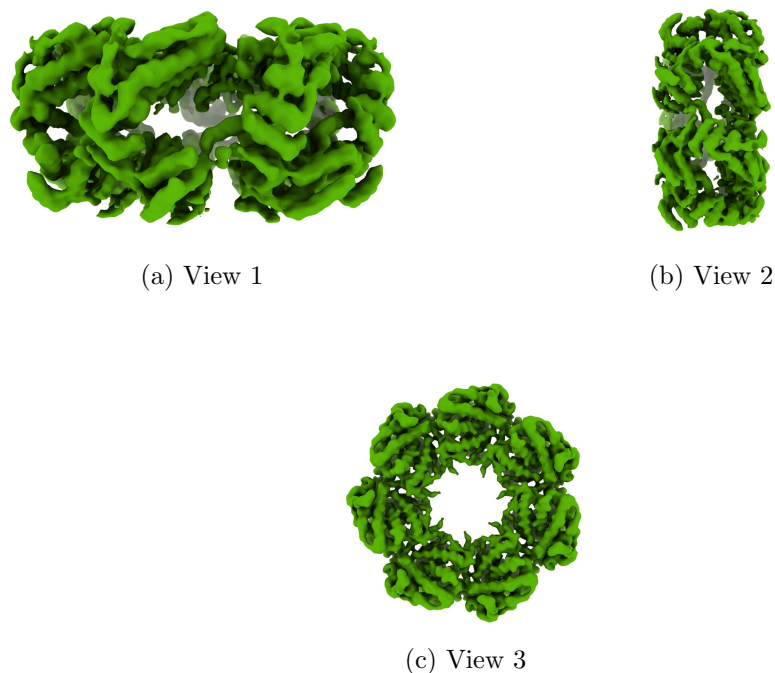
Figure 4: Isosurface at threshold=1.070000. Views generated by ChimeraX at a the following X, Y, Z angles: View 1 (0, -90, -90), View 2 (-90, 0, -90), View 3 (0, 0, 0).
