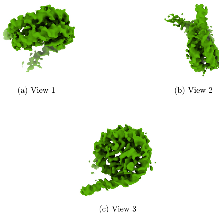
Figure 4: Isosurface at threshold=0.013200. Views generated by ChimeraX at a the following X, Y, Z angles: View 1 (0, -90, -90), View 2 (-90, 0, -90), View 3 (0, 0, 0).
