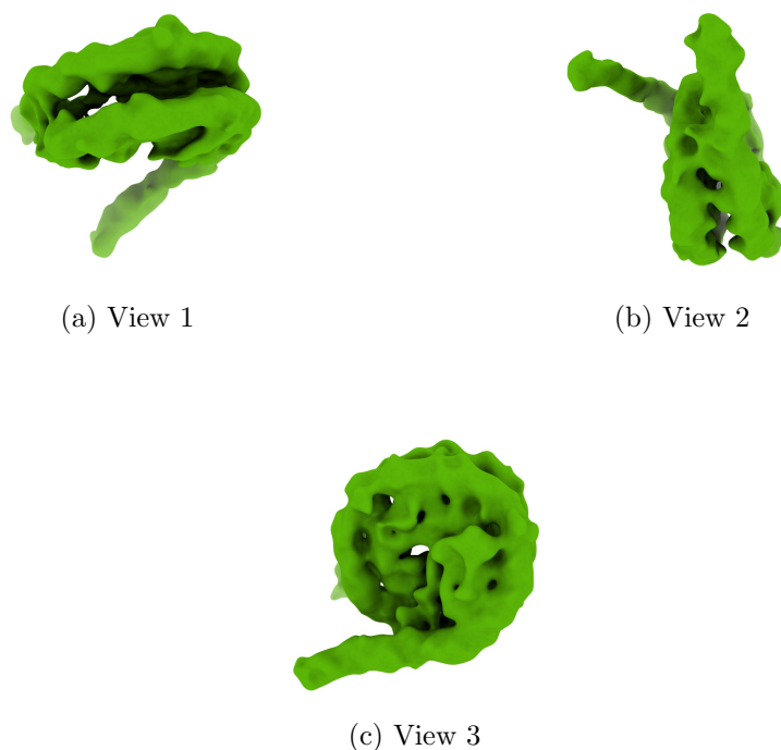
Figure 4: Isosurface at threshold=0.009410. Views generated by ChimeraX at a the following X, Y, Z angles: View 1 (0, -90, -90), View 2 (-90, 0, -90), View 3 (0, 0, 0).
