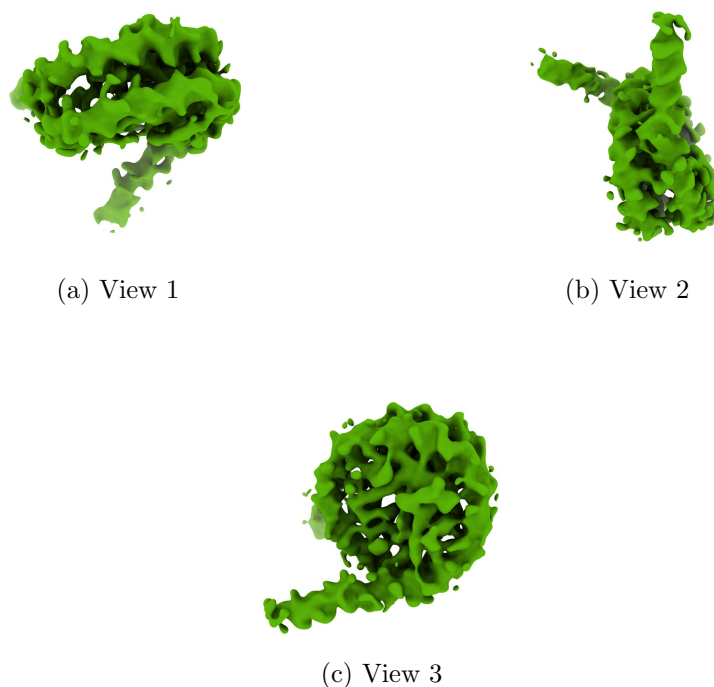
Figure 4: Isosurface at threshold=0.013700. Views generated by ChimeraX at a the following X, Y, Z angles: View 1 (0, -90, -90), View 2 (-90, 0, -90), View 3 (0, 0, 0).
