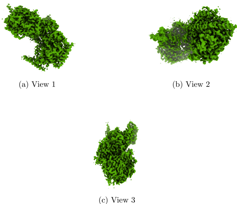
Figure 4: Isosurface at threshold=0.033500. Views generated by ChimeraX at a the following X, Y, Z angles: View 1 (0, -90, -90), View 2 (-90, 0, -90), View 3 (0, 0, 0).
