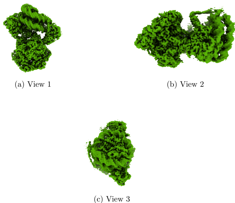
Figure 4: Isosurface at threshold=0.196000. Views generated by ChimeraX at a the following X, Y, Z angles: View 1 (0, -90, -90), View 2 (-90, 0, -90), View 3 (0, 0, 0).
