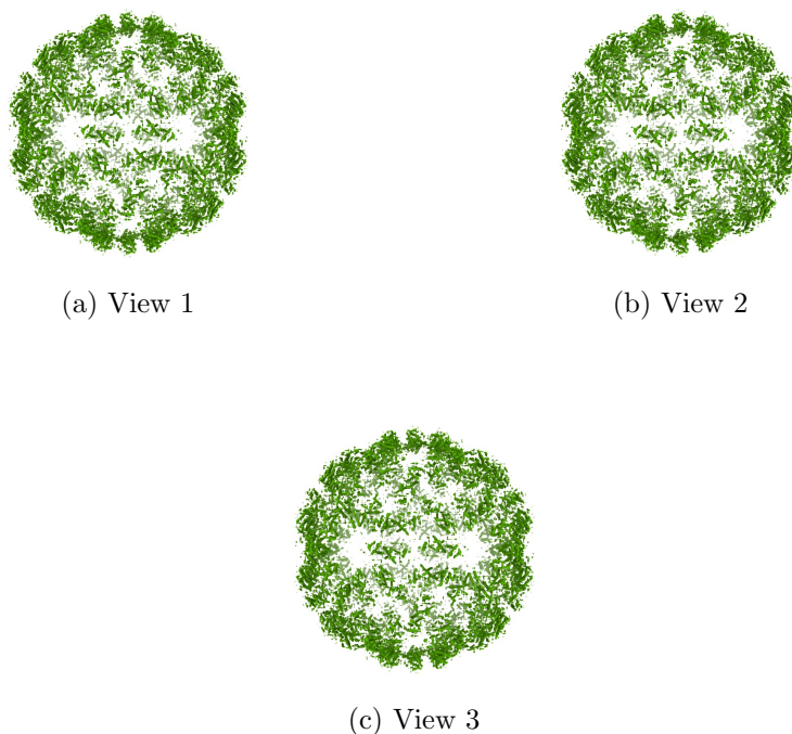
Figure 4: Isosurface at threshold=0.177000. Views generated by ChimeraX at a the following X, Y, Z angles: View 1 (0, -90, -90), View 2 (-90, 0, -90), View 3 (0, 0, 0).
