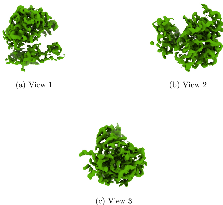
Figure 4: Isosurface at threshold=2.740000. Views generated by ChimeraX at a the following X, Y, Z angles: View 1 (0, -90, -90), View 2 (-90, 0, -90), View 3 (0, 0, 0).
