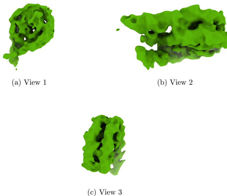
Figure 4: Isosurface at threshold=0.007420. Views generated by ChimeraX at a the following X, Y, Z angles: View 1 (0, -90, -90), View 2 (-90, 0, -90), View 3 (0, 0, 0).
