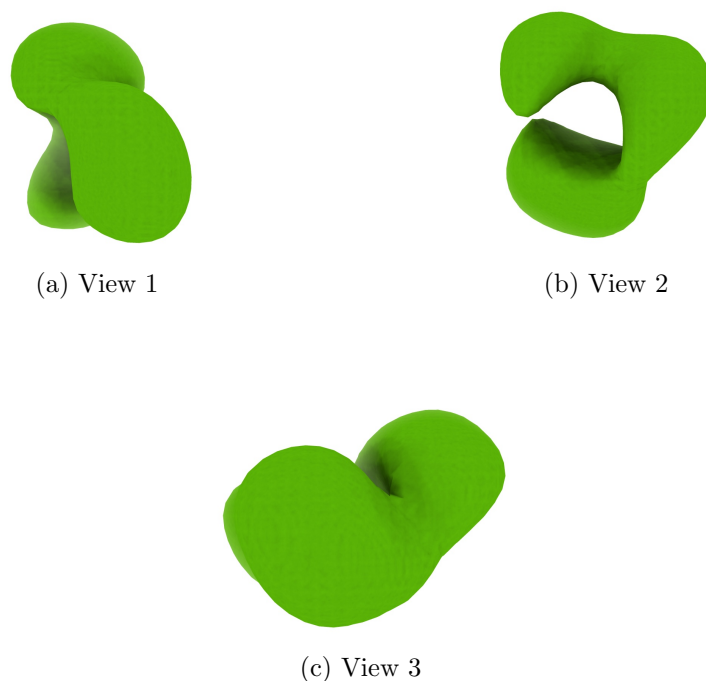
Figure 4: Isosurface at threshold=0.049700. Views generated by ChimeraX at a the following X, Y, Z angles: View 1 (0, -90, -90), View 2 (-90, 0, -90), View 3 (0, 0, 0).
