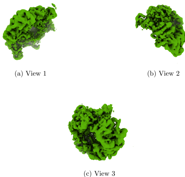
Figure 4: Isosurface at threshold=0.147000. Views generated by ChimeraX at a the following X, Y, Z angles: View 1 (0, -90, -90), View 2 (-90, 0, -90), View 3 (0, 0, 0).
