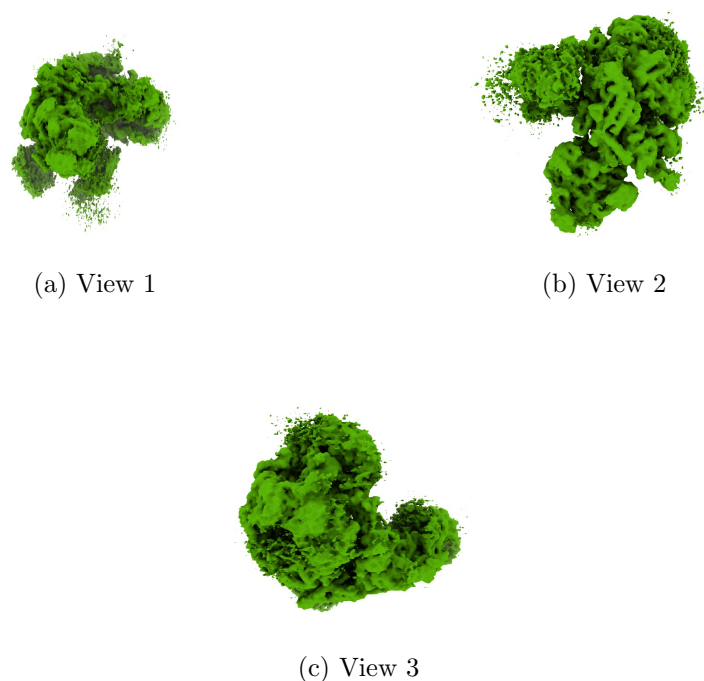
Figure 4: Isosurface at threshold=1.430000. Views generated by ChimeraX at a the following X, Y, Z angles: View 1 (0, -90, -90), View 2 (-90, 0, -90), View 3 (0, 0, 0).
