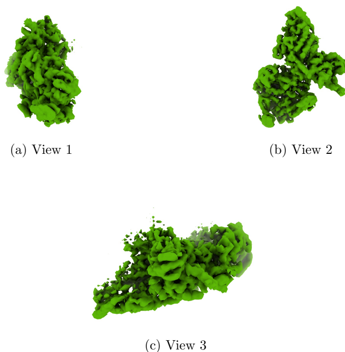
Figure 4: Isosurface at threshold=0.172000. Views generated by ChimeraX at a the following X, Y, Z angles: View 1 (0, -90, -90), View 2 (-90, 0, -90), View 3 (0, 0, 0).
