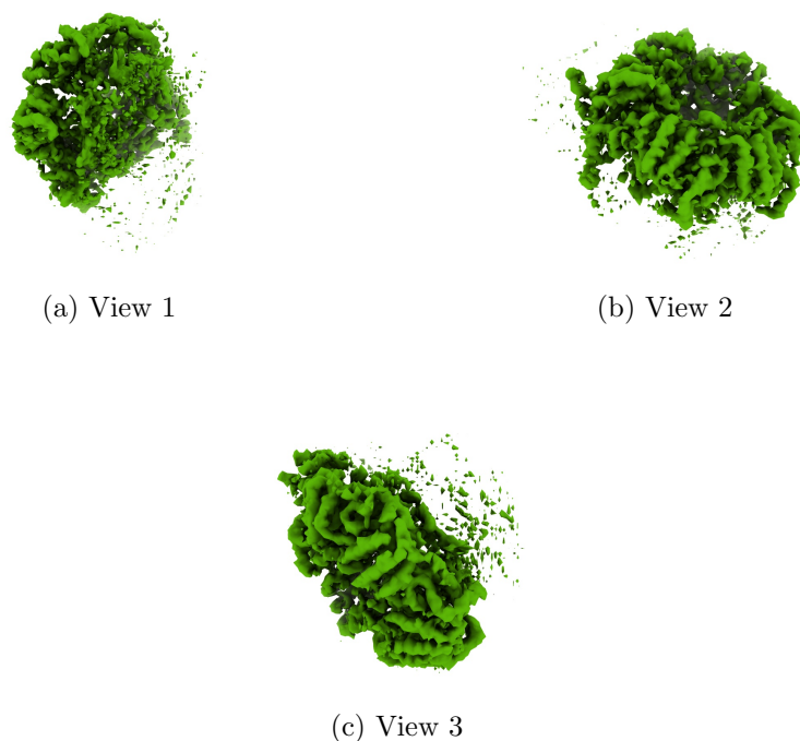
Figure 4: Isosurface at threshold=0.358000. Views generated by ChimeraX at a the following X, Y, Z angles: View 1 (0, -90, -90), View 2 (-90, 0, -90), View 3 (0, 0, 0).
