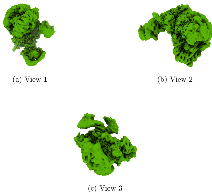
Figure 4: Isosurface at threshold=0.137000. Views generated by ChimeraX at a the following X, Y, Z angles: View 1 (0, -90, -90), View 2 (-90, 0, -90), View 3 (0, 0, 0).
