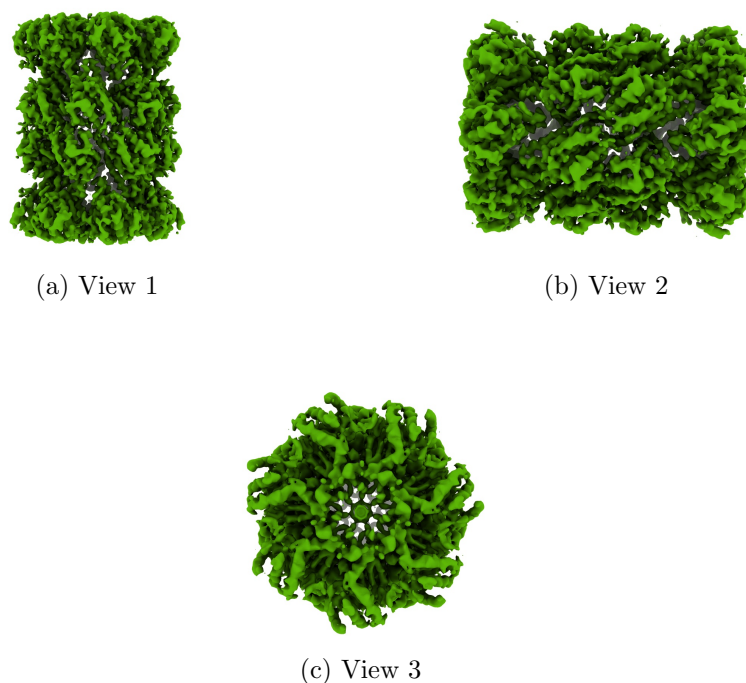
Figure 4: Isosurface at threshold=0.422000. Views generated by ChimeraX at the following X, Y, Z angles: View 1 (0, -90, -90), View 2 (-90, 0, -90), View 3 (0, 0, 0).
