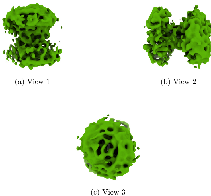
Figure 4: Isosurface at threshold=0.086800. Views generated by ChimeraX at a the following X, Y, Z angles: View 1 (0, -90, -90), View 2 (-90, 0, -90), View 3 (0, 0, 0).
