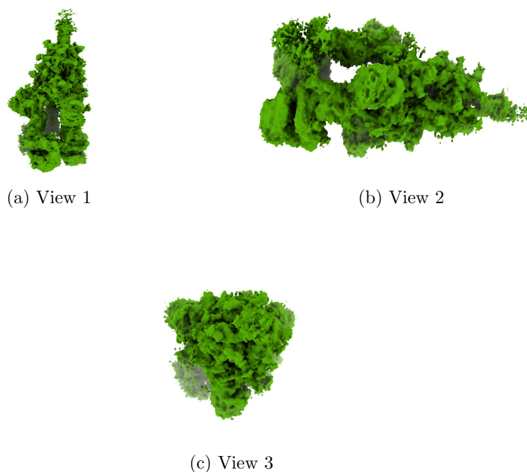
Figure 4: Isosurface at threshold=0.082400. Views generated by ChimeraX at a the following X, Y, Z angles: View 1 (0, -90, -90), View 2 (-90, 0, -90), View 3 (0, 0, 0).
