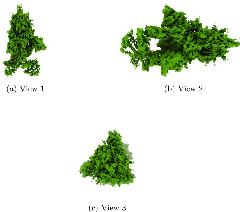
Figure 4: Isosurface at threshold=0.077500. Views generated by ChimeraX at a the following X, Y, Z angles: View 1 (0, -90, -90), View 2 (-90, 0, -90), View 3 (0, 0, 0).
