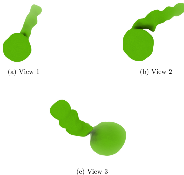
Figure 4: Isosurface at threshold=0.019200. Views generated by ChimeraX at a the following X, Y, Z angles: View 1 (0, -90, -90), View 2 (-90, 0, -90), View 3 (0, 0, 0).
