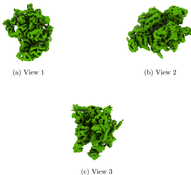
Figure 4: Isosurface at threshold=0.095000. Views generated by ChimeraX at a the following X, Y, Z angles: View 1 (0, -90, -90), View 2 (-90, 0, -90), View 3 (0, 0, 0).
