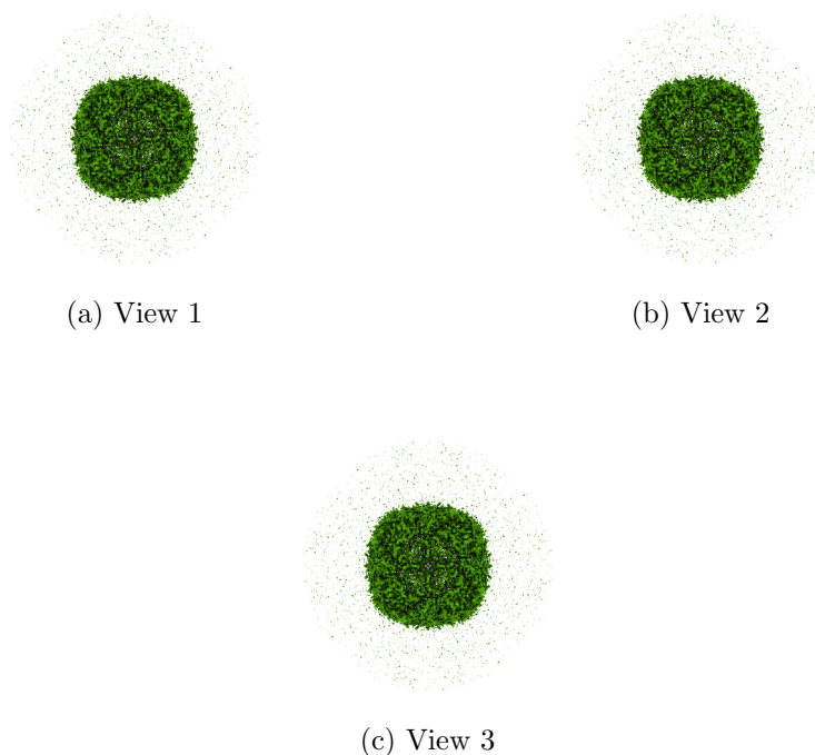
Figure 4: Isosurface at threshold=0.077000. Views generated by ChimeraX at a the following X, Y, Z angles: View 1 (0, -90, -90), View 2 (-90, 0, -90), View 3 (0, 0, 0).
