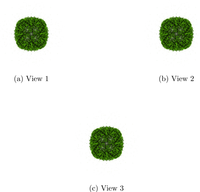
Figure 4: Isosurface at threshold=0.077000. Views generated by ChimeraX at a the following X, Y, Z angles: View 1 (0, -90, -90), View 2 (-90, 0, -90), View 3 (0, 0, 0).
