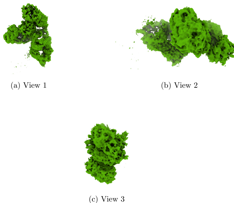
Figure 4: Isosurface at threshold=0.062100. Views generated by ChimeraX at a the following X, Y, Z angles: View 1 (0, -90, -90), View 2 (-90, 0, -90), View 3 (0, 0, 0).
