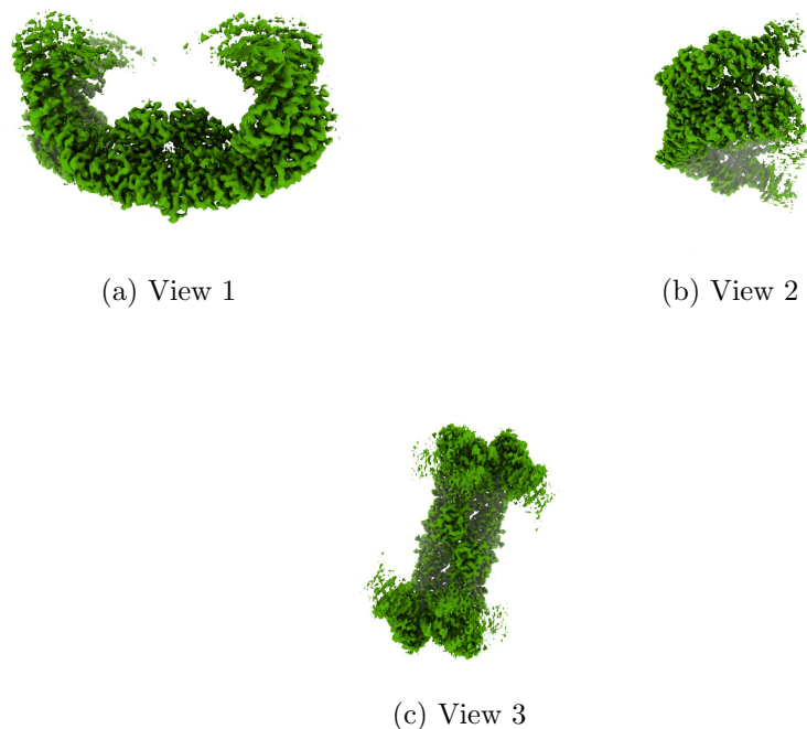
Figure 4: Isosurface at threshold=0.011780. Views generated by ChimeraX at a the following X, Y, Z angles: View 1 (0, -90, -90), View 2 (-90, 0, -90), View 3 (0, 0, 0).
