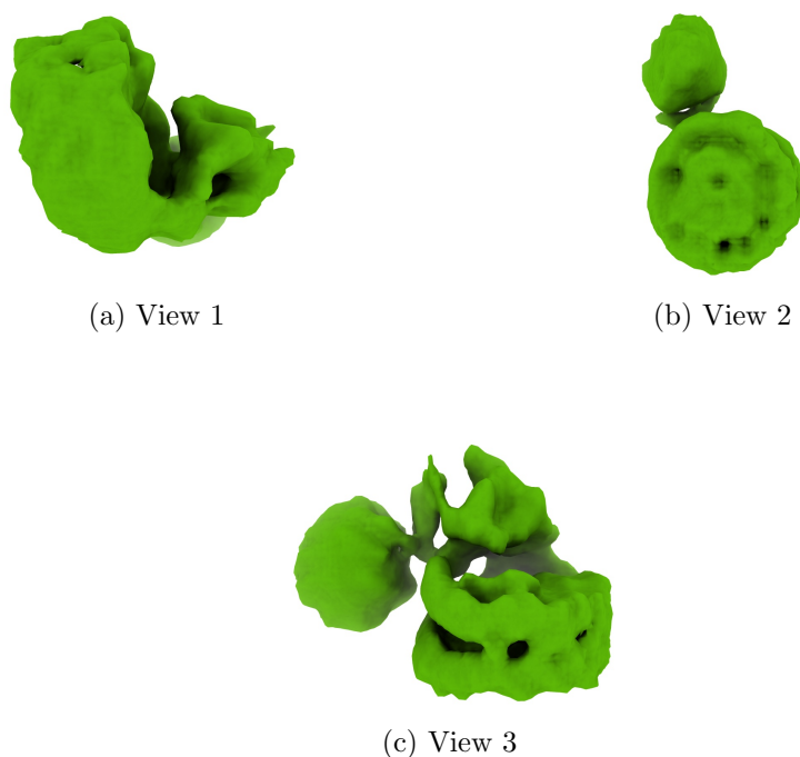
Figure 4: Isosurface at threshold=0.050500. Views generated by ChimeraX at a the following X, Y, Z angles: View 1 (0, -90, -90), View 2 (-90, 0, -90), View 3 (0, 0, 0).
