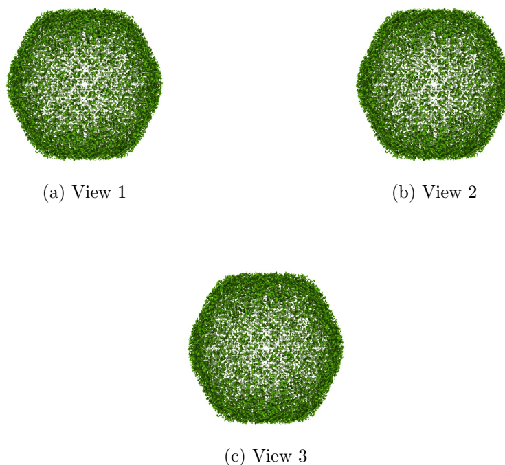
Figure 4: Isosurface at threshold=0.214000. Views generated by ChimeraX at a the following X, Y, Z angles: View 1 (0, -90, -90), View 2 (-90, 0, -90), View 3 (0, 0, 0).
