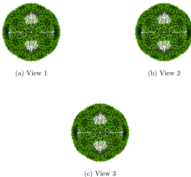
Figure 4: Isosurface at threshold=0.273000. Views generated by ChimeraX at a the following X, Y, Z angles: View 1 (0, -90, -90), View 2 (-90, 0, -90), View 3 (0, 0, 0).
