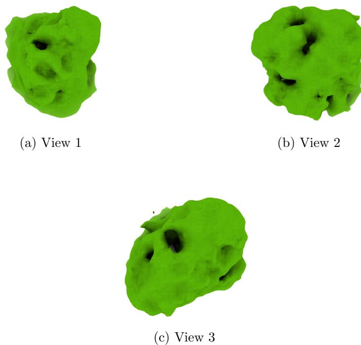
Figure 4: Isosurface at threshold=1.950000. Views generated by ChimeraX at a the following X, Y, Z angles: View 1 (0, -90, -90), View 2 (-90, 0, -90), View 3 (0, 0, 0).
